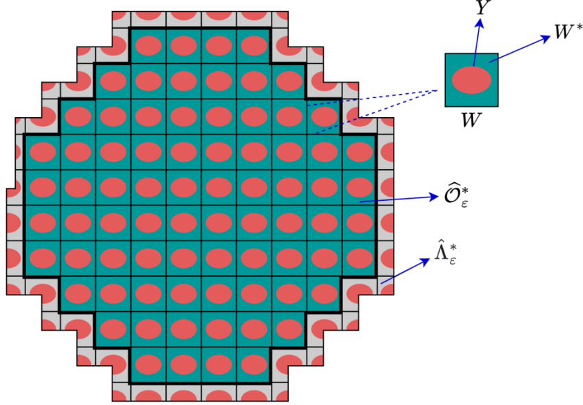
Figure 1: The Perforated domain \mathcal{O}_\varepsilon^* and the reference cell W .
